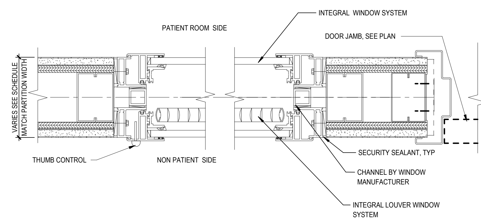
(A1) WINDOW W/ INTEGRAL LOUVER JAMB 3" = 1'-0"
