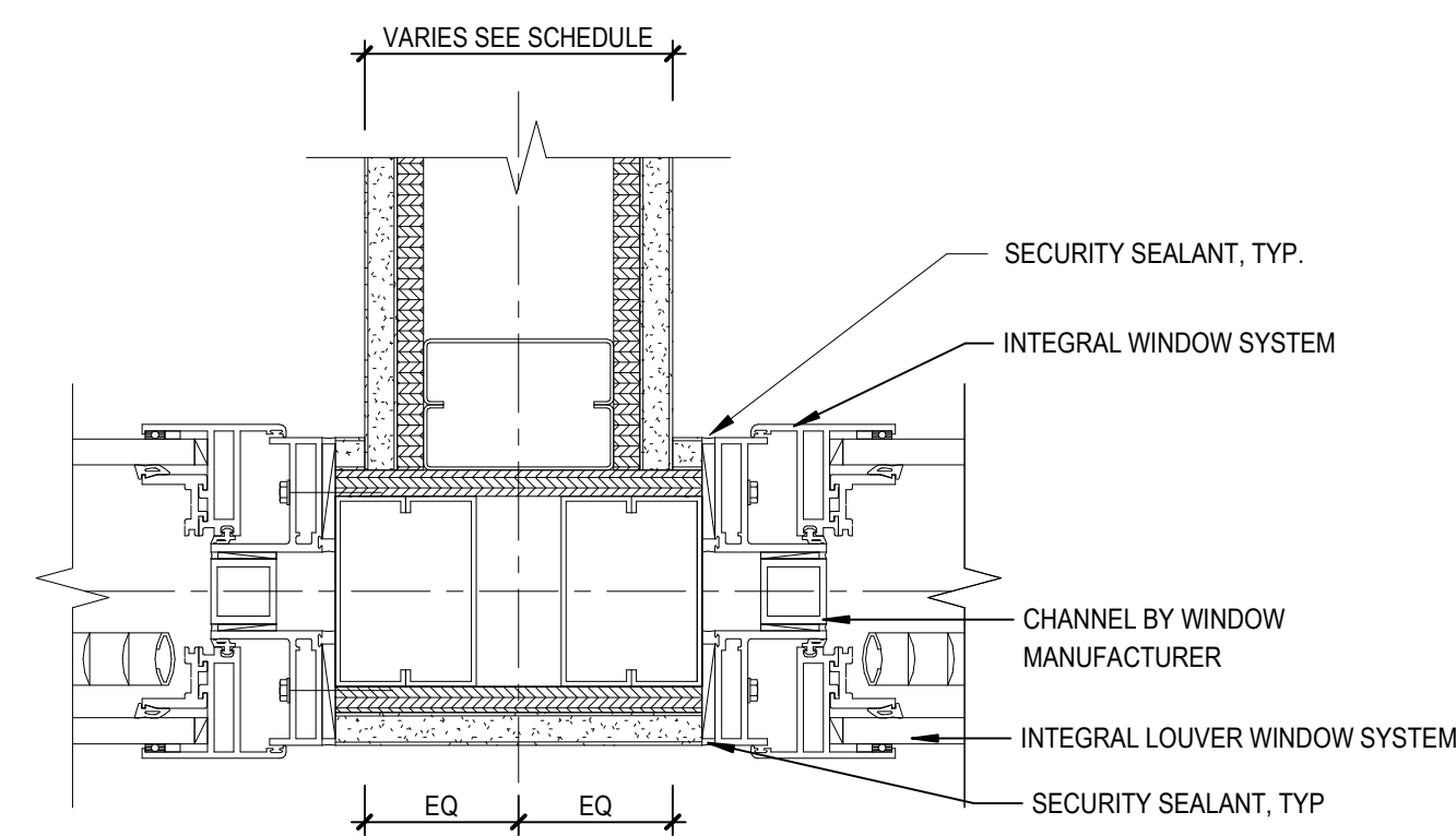
B1 WINDOW W/ INTEGRAL LOUVER @CORNER 3" = 1'-0"
