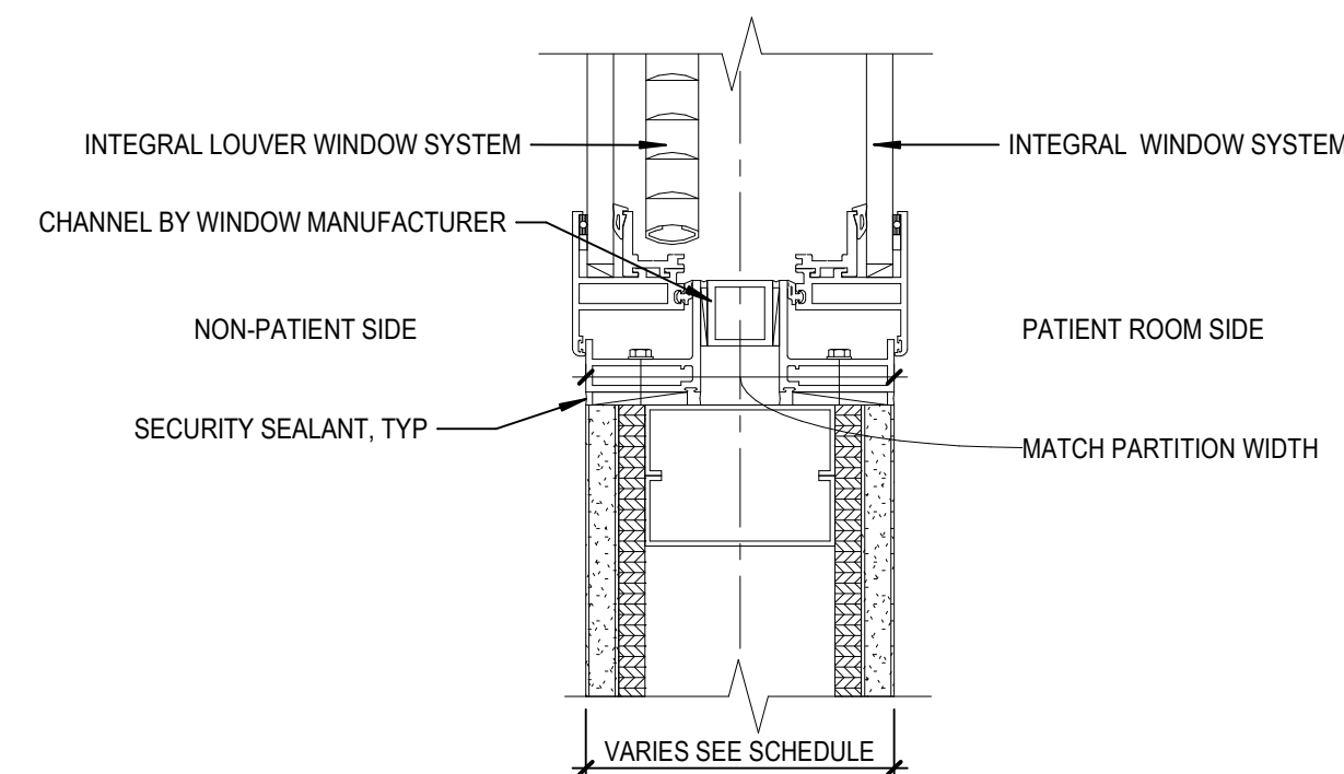
A2 WINDOW W/ INTEGRAL LOUVER HEAD-SILL SIM 3" = 1'-0"
