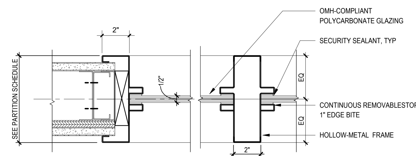
C2 HM WINDOW JAMB- BH
